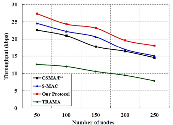
Fig. 11. Comparison of throughput for different number of nodes.
