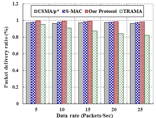
Fig. 16. Comparison of packet delivery ratio for different data rates.
