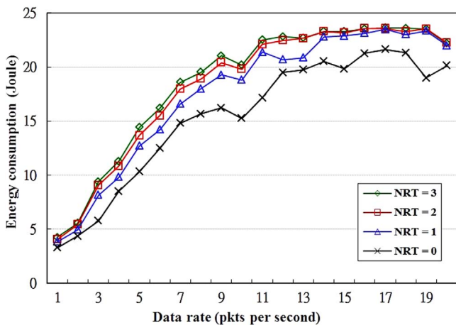
Fig. 9. Energy consumption for different values of NRT.
