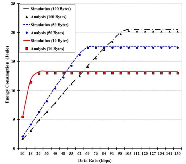
Fig. 6. Validation of energy consumption for different data rates.
