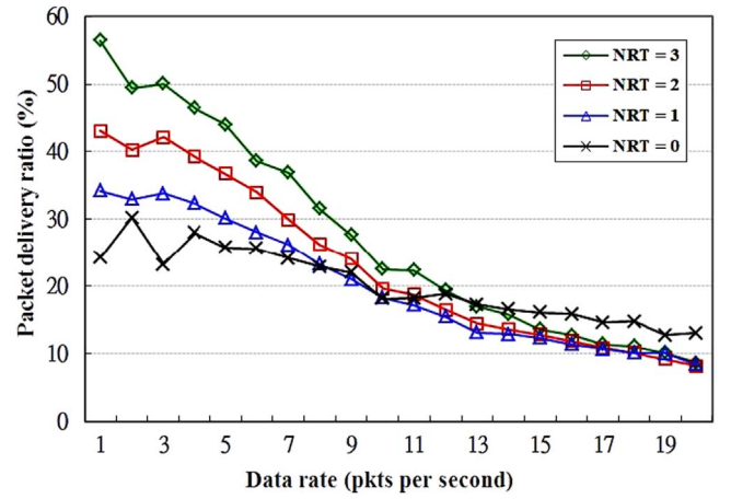
Fig. 10. Packet delivery ratio for different values of NRT.
