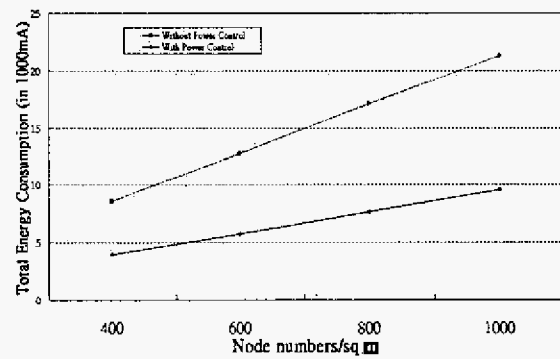
Figure 8: Total energy consumption for different node numbers with and without power control.
