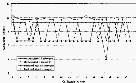
Figure 10: Average network lifetime for different configurations with different node densities.
