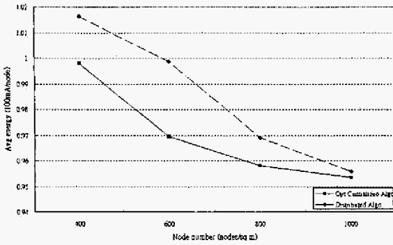
Figure 6: Average energy consumption for different node numbers with transmission power control.
